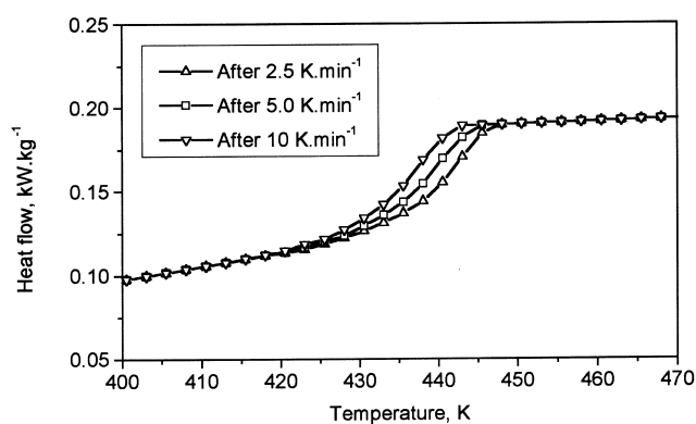
Fig. 6. Second scans of DGEBA–mPDA samples reacted at different dT/dr .
